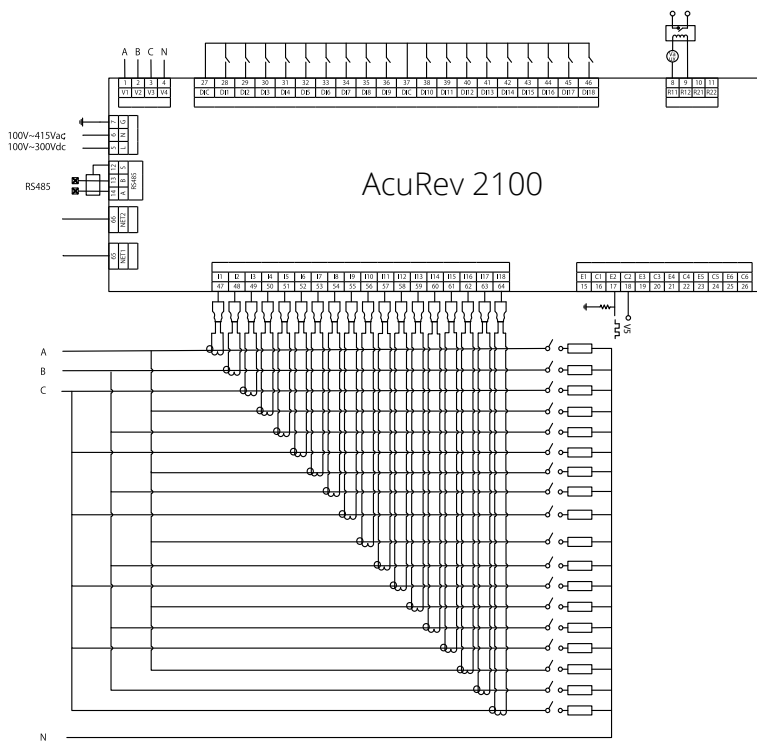
Fig. 2-8 Single Phase
