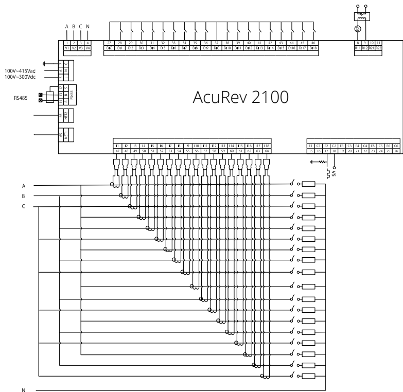
Fig. 2-9 3-Phase 4-Wire
