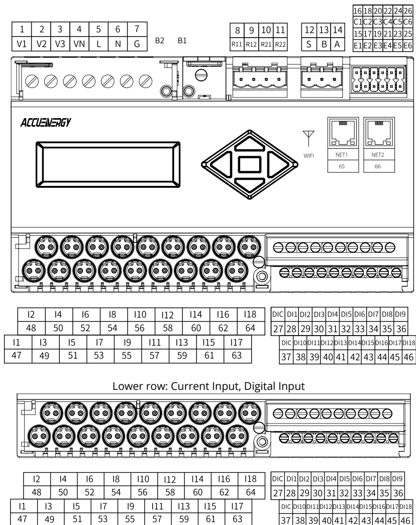
Fig. 2-6 AcuRev 2100 Terminals
